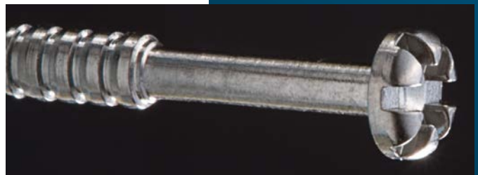
Implantable pacing component – Titanium; machined complete, including deburring, on 4-axis Swiss lathe.
